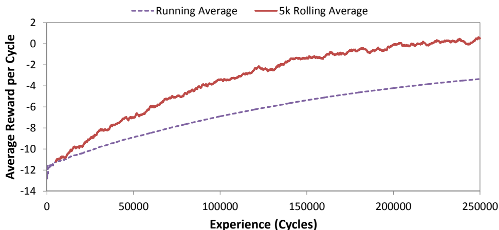
Figure 10: Online performance on a challenging domain
