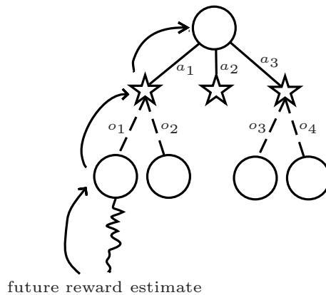
Figure 1: A \rho UCT search tree
